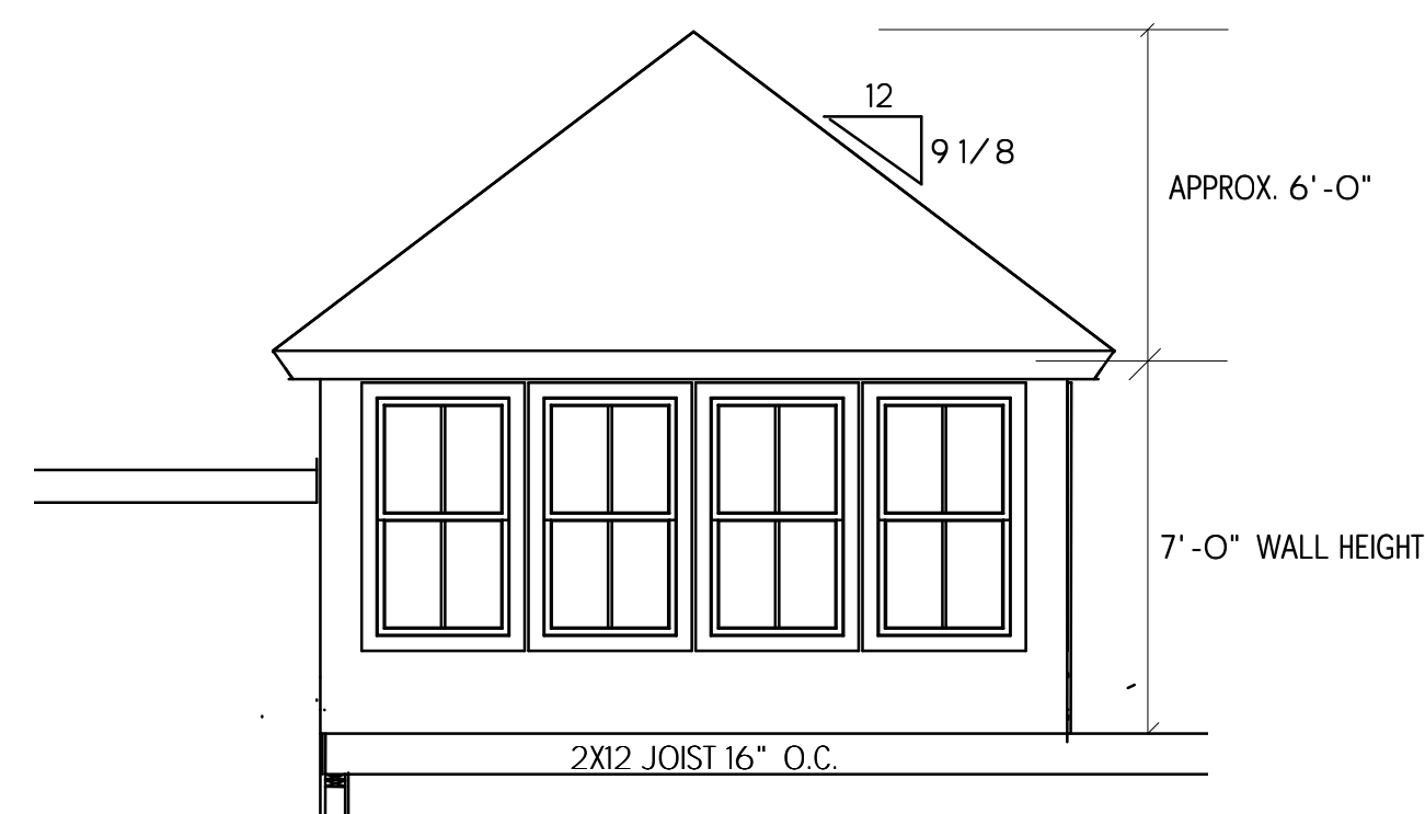
WESTERLY ELEVATION
